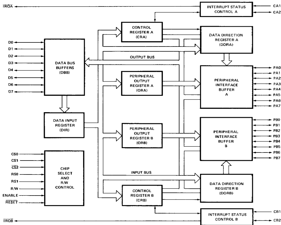
Figure 3. SY6520 Block Diagram
