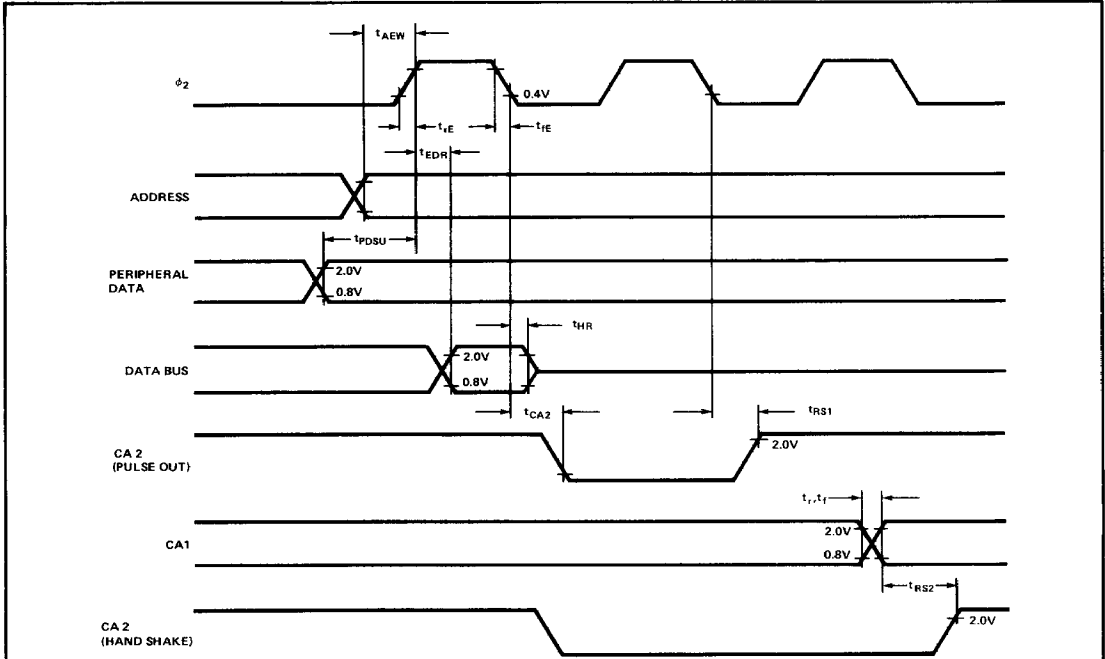
Figure 1. Read Timing Characteristics
