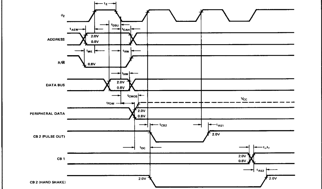
Figure 2. Write Timing Characteristics
