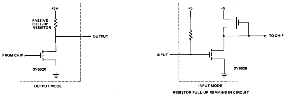
Figure 6. Port A Buffer Circuit (PA 0 -PA 7 )
