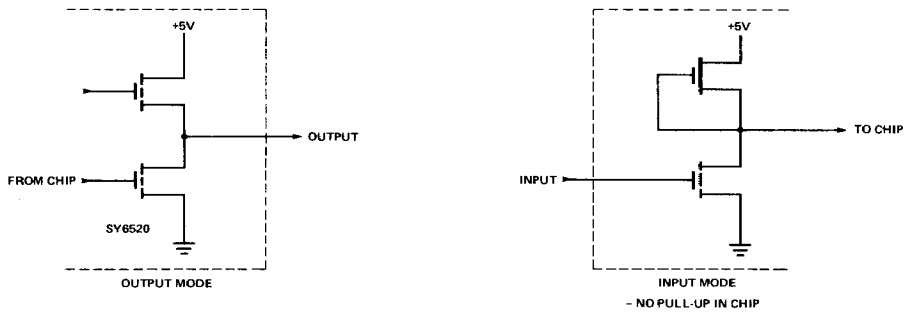
Figure 7. Port B Buffer Circuit (PB 0 -PB 7 )
