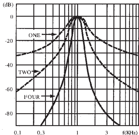
Figure 18 : Frequency Response of Bandpass Filter
