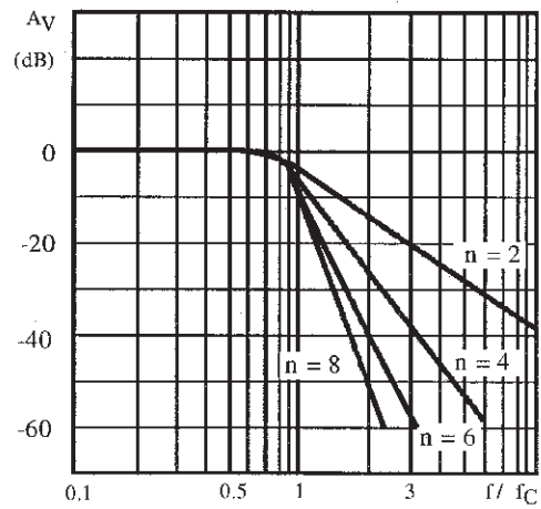
Figure 10 : Amplitude Response
