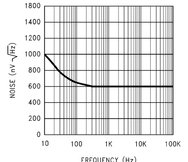
Noise Voltage
