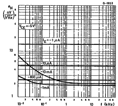
Equivalent Input Noise Voltage (for BCY71 only).
