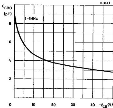
Collector-base Capacitance.
