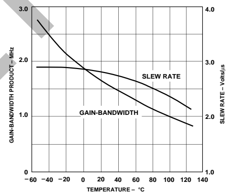
Figure 21. Gain-Bandwidth Product and Slew Rate vs. Temperature
